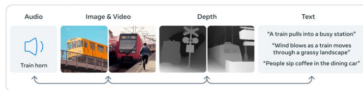
Embedding-space arithmetic
